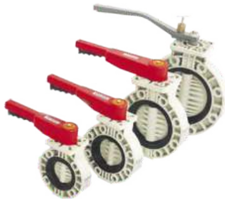
PP BUTTERFLY VALVES SIZES AVAILABLE: 2", 3", 4", 6" & 8"
